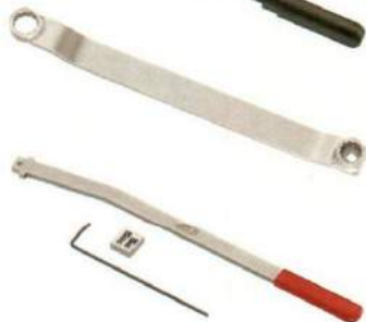
4232 FORD, MAZDA 惰輪皮帶調整 扳手(TDCI) FORD, MAZDA SERPENTINE BELT TOOL(TDCI)
